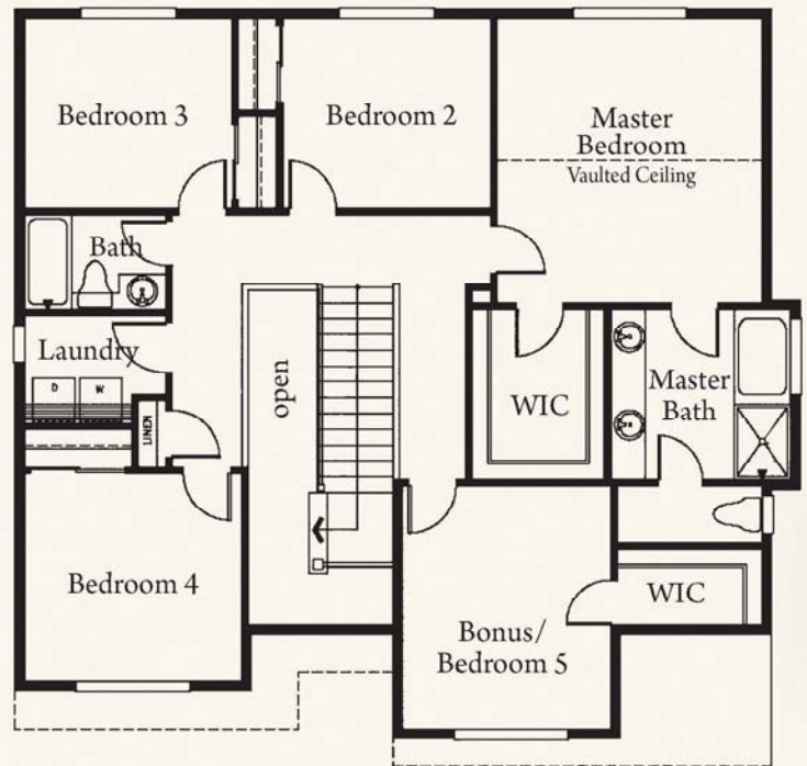
UPPER FLOOR
